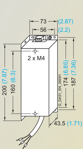
EMC filter for frame size A
